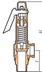
N9LS Type Lever 1/2"~2"
